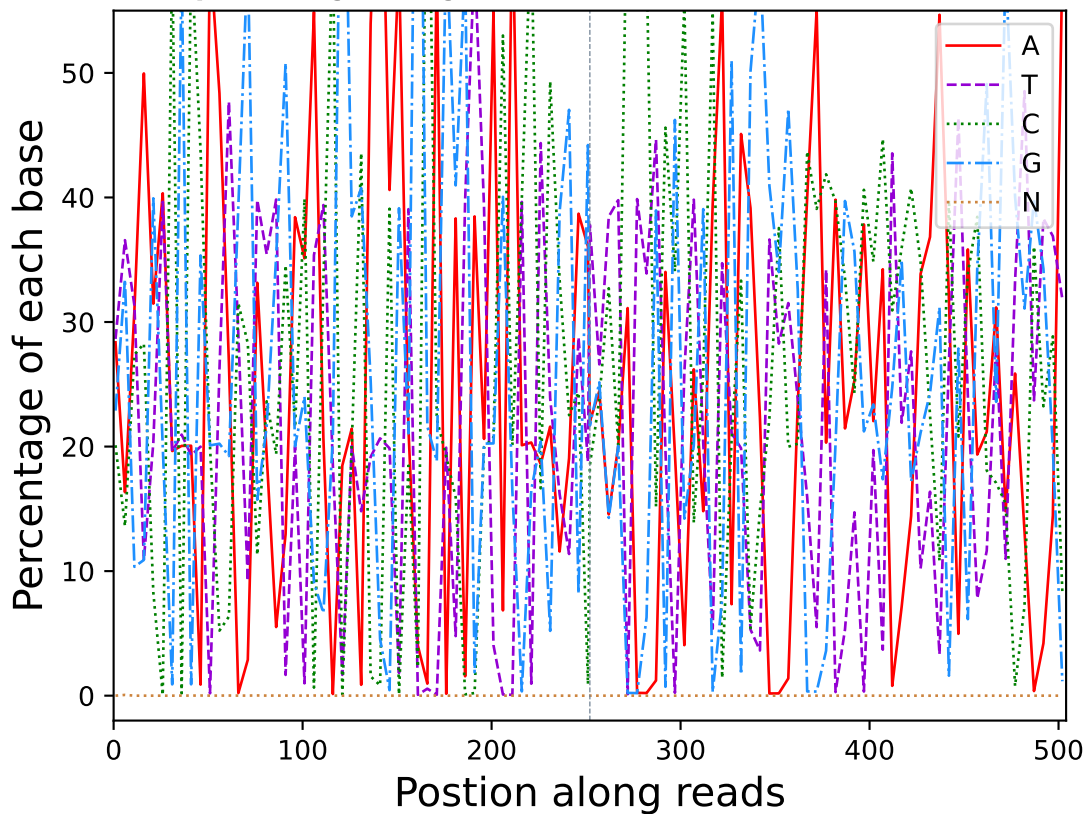
Base percentage along reads (R10921)
